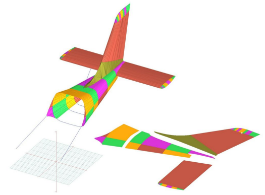
Tecnam P2008 Empennage Cover, 3D model
